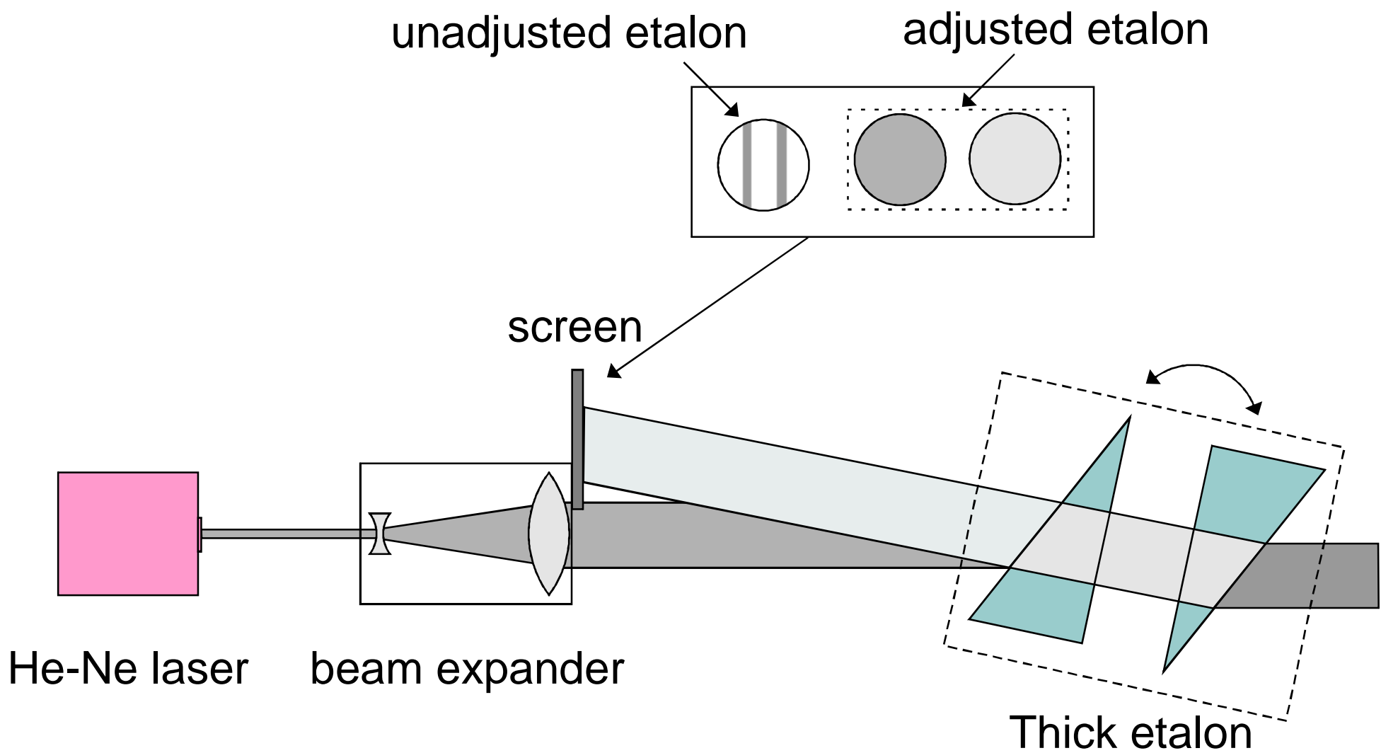
The checking of the thick etalon adjustment
